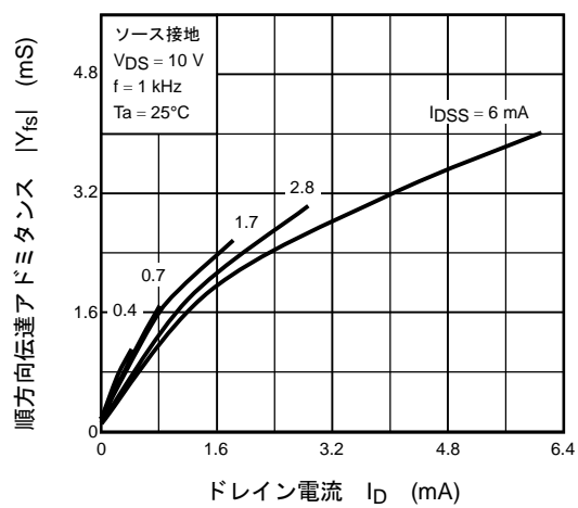
|Yfs| - ID
